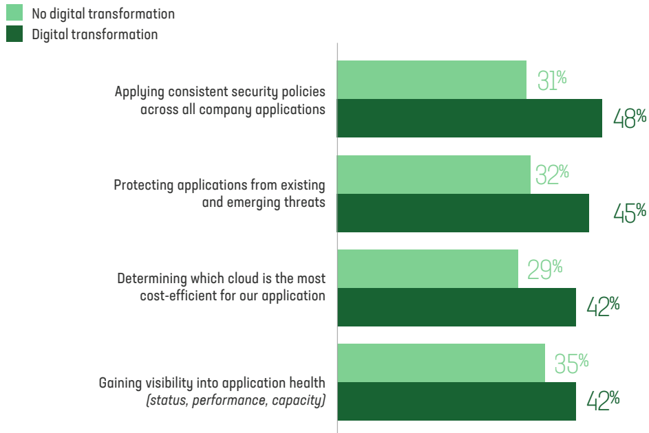
FIGURE 03: MULTI-CLOUD CHALLENGES
